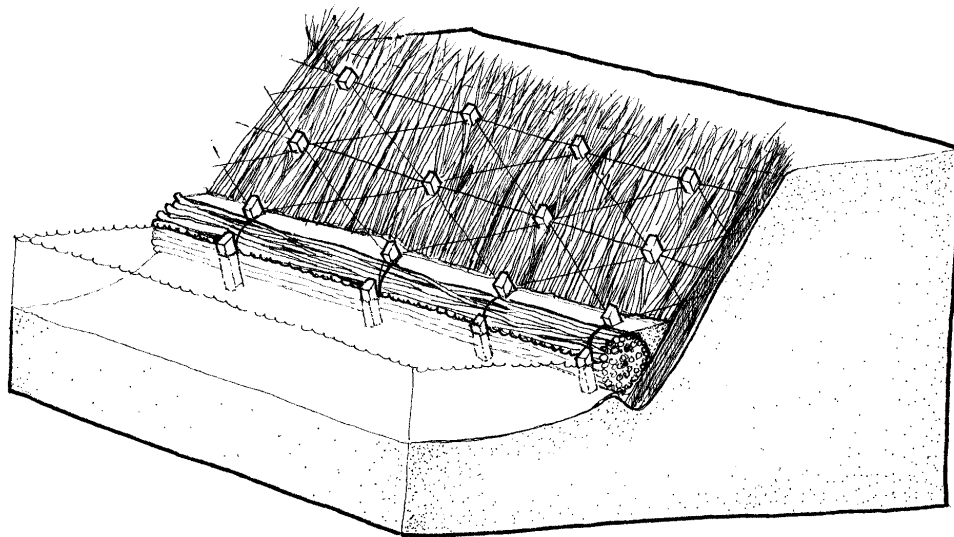
Brush Mattress
