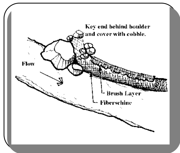
Fig. 3.8 Endpoint Protection
